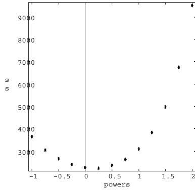
Fig. 6. Box-Cox power plot
